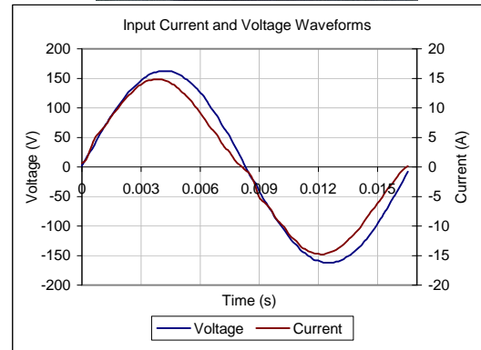
Input AC Current Waveform (ITHD = 8.73%, 50% Load)
