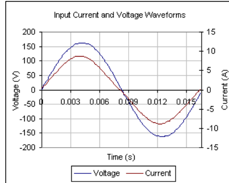
Input AC Current Waveform ( I_{THD} = 10.2\% , 50% Load)
